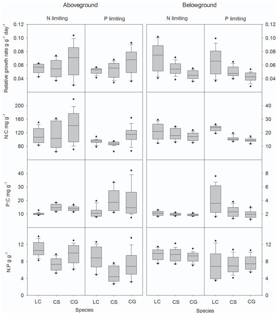
Figure 5. Variation of relative growth rate, N:C, P:C and N:P across the three species. doi:10.1371/journal.pone.0032162.g005
