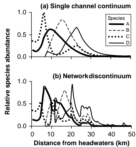
Fig. 10 Distributions of four hypothetical species (see Fig. 9) along the downstream profile based on predicted Hynsite and Forsite concentrations (see Fig. 8).
