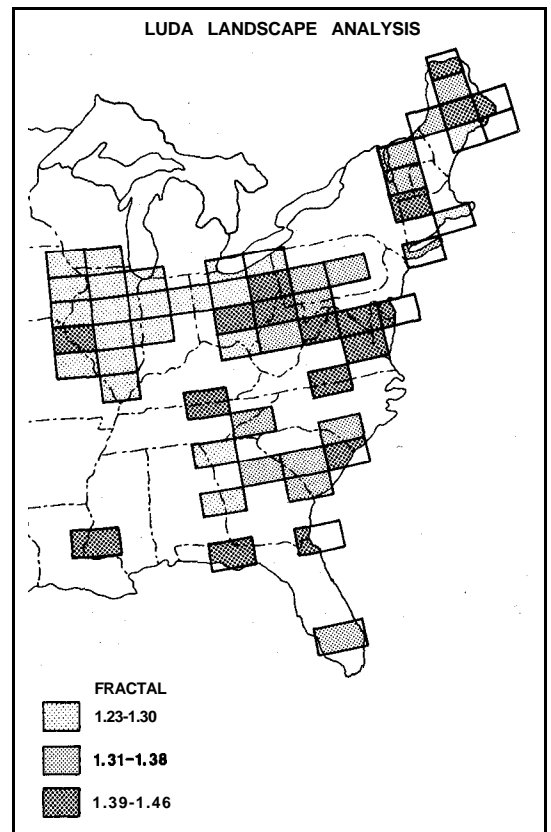
Fig. 3. Geographic distribution of the fractal dimension, D_2 (Equation 3).
